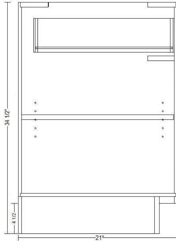
SIDE VIEW
