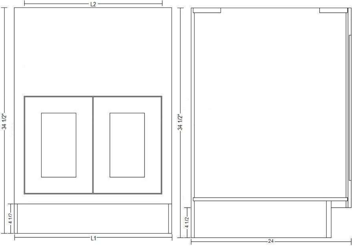
SIDE VIEW
