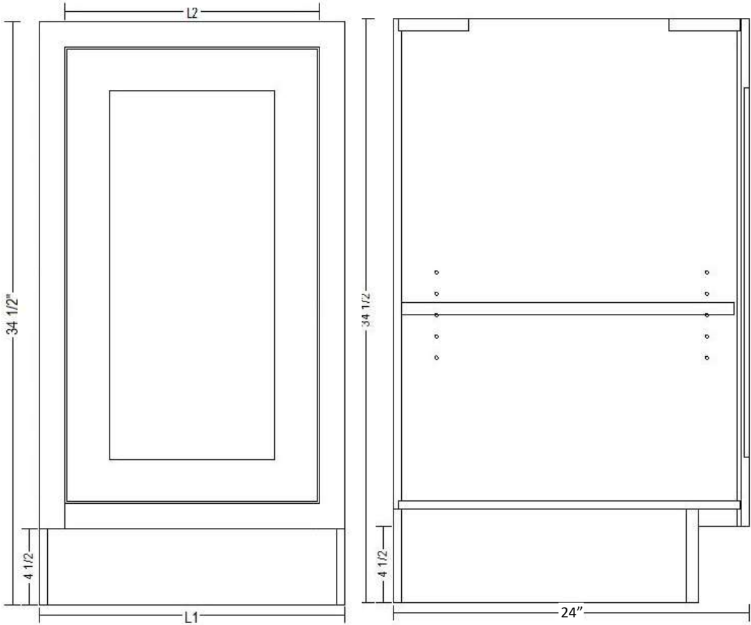
FRONT VIEW
